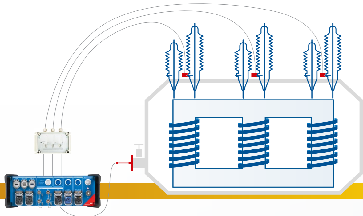
The MONTESTO 200 PD measurement and temporary monitoring system can be easily connected to permanently-installed bushing tap sensors via a terminal box. This enables a safe and convenient plug-and-play set up when power transformers are on line.
