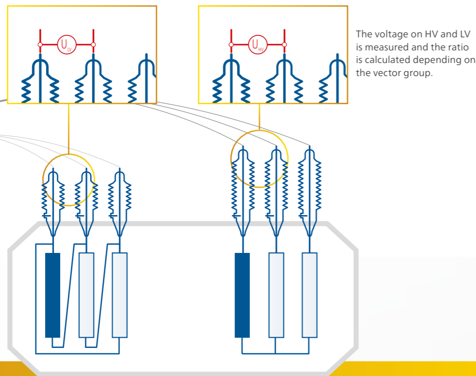
TESTRANO 600, as well as CPC 100 + CP SB1, allows transformer turns ratio measurements of power transformers with no additional need for rewiring.
