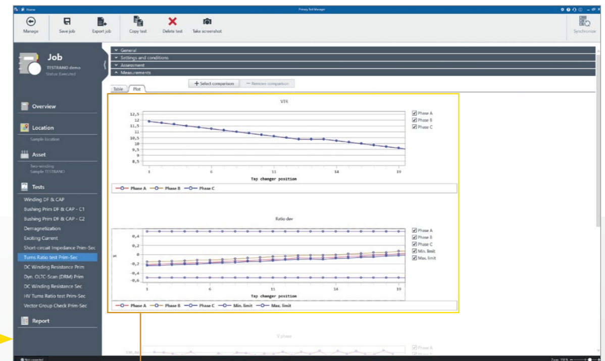
The TTR is measured for all three phases at each tap position. According to international standards the results should not deviate more than 0,5 % from the nominal nameplate values.
