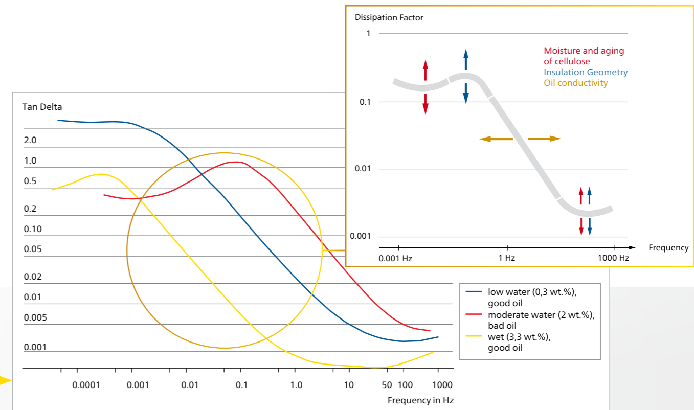
The dielectric response curve allows conclusions to be drawn about the different factors that influence the measurement result.
