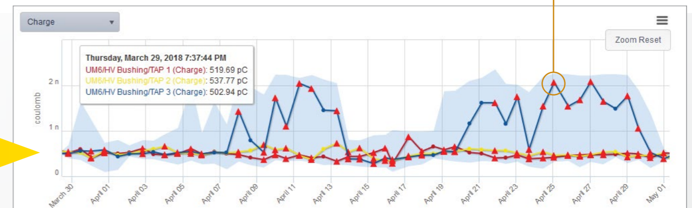
PD trend charts for each phase or channel. Scrolling over points displays PD values. Users can zoom in to see more detail.
