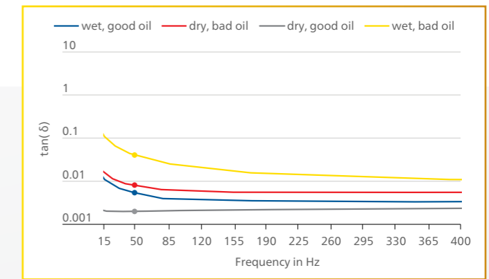
The \tan(\delta) of four different transformers below and above line frequency (50 Hz).
