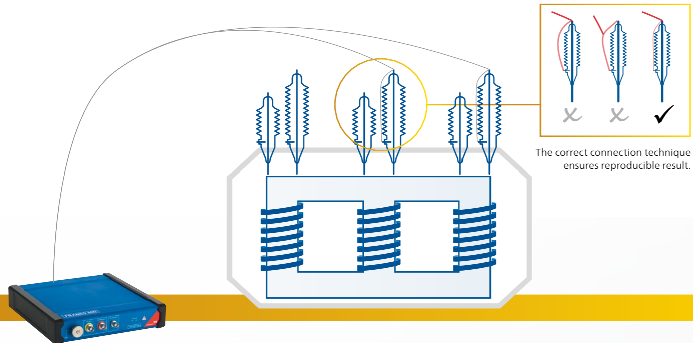
FRANEO 800 allows reliable core and windings diagnosis of power transformers by using sweep frequency response analysis (SFRA).
