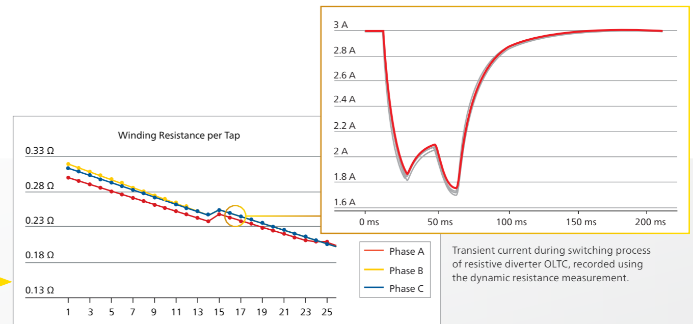
Winding resistance per tap, recorded using the static winding resistance measurement.
