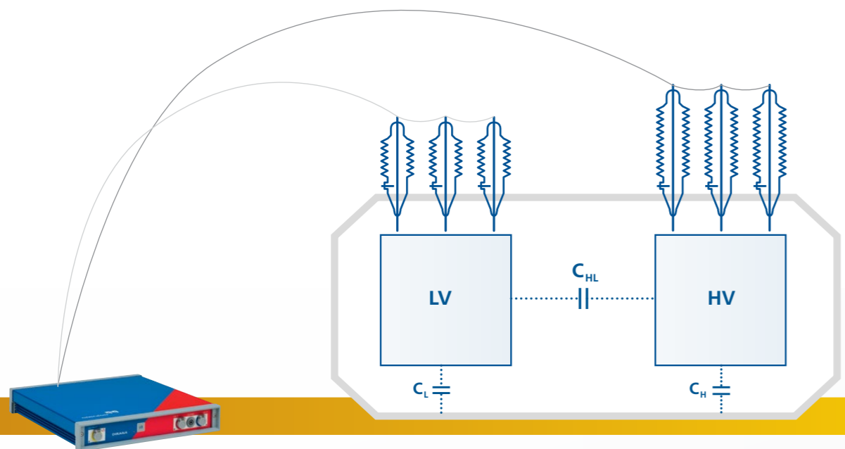
DIRANA determines the moisture content of oil-paper insulated power transformers and also assesses the condition of bushings by using dielectric response analysis.
