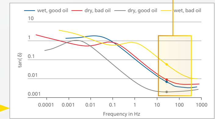
Depending on the test device, different frequency ranges can be measured, e.g. from 15 Hz to 400 Hz with TESTRANO 600 and from 10 \mu Hz to 5 kHz with DIRANA.
