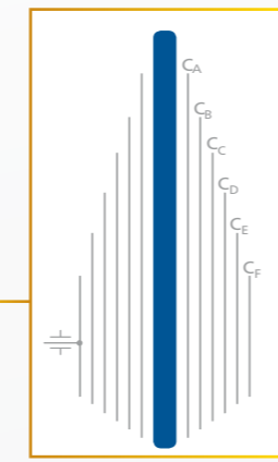
The capacitive layers of a bushing
