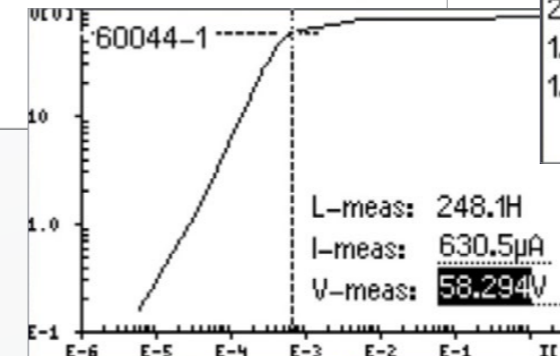
Different test cards support you in checking and assessing relevant CT parameters such as ratio, resistance and its protection class.
